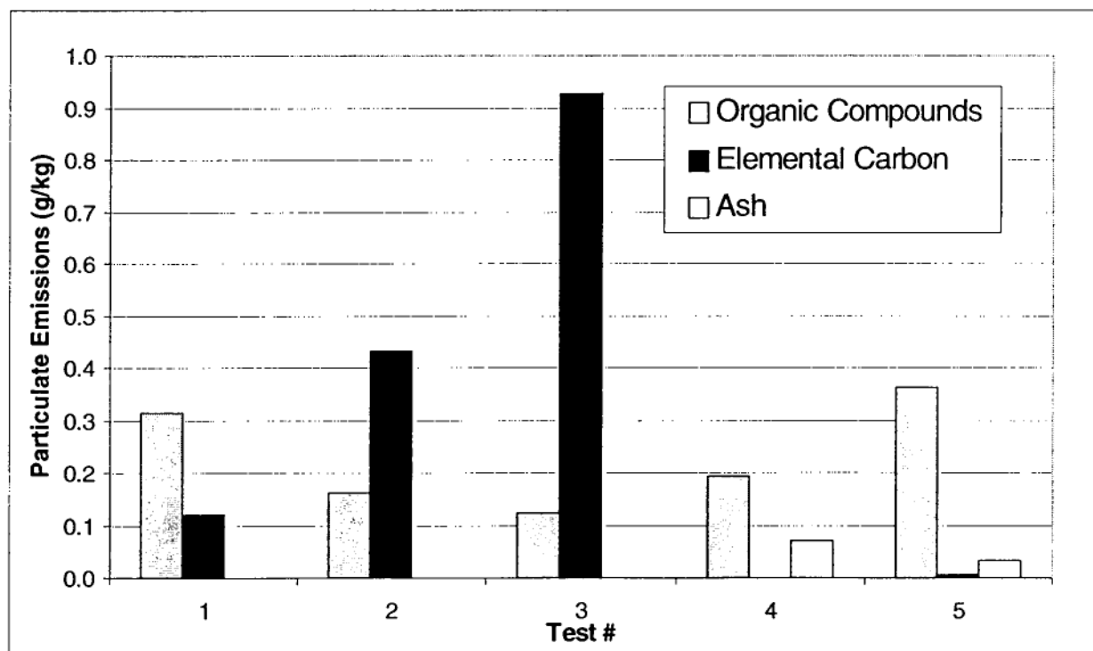
Figure 2. Composition of PM emissions. Tests 1, 2, & 3 are for a top-feed model burning softwood pellets at 0.72, 1.46, and 2.45 kg/hr. Tests 4 & 5 are for an under-feed model. Softwood pellets at 1.55 kg/hr were burned in test 4. Hardwood pellets at 1.55 kg/hr were burned in test 5.
