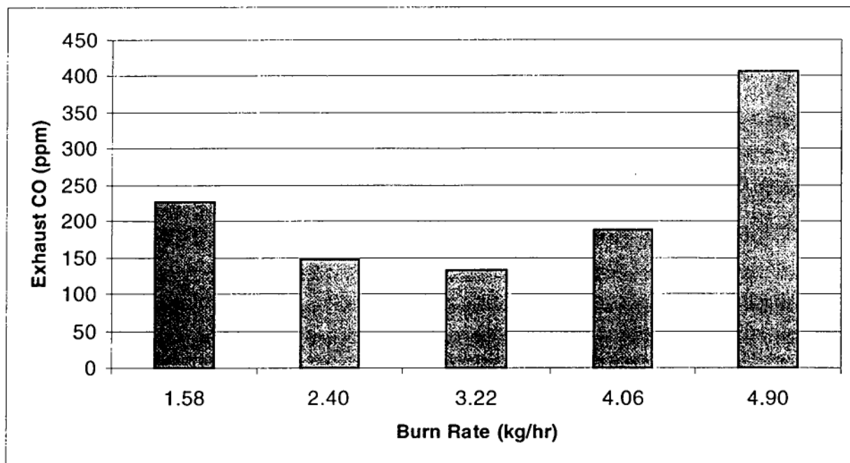
Figure 1. Carbon monoxide concentration in exhaust gas versus burn rate with a new top-feed pellet stove model burning softwood pellets.
